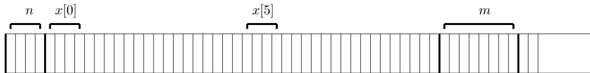
Figure 2.1: The layout of memory on the stack for the declaration above.
