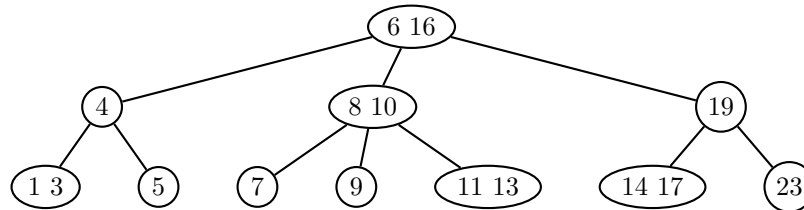
Figure 25.14: After 16 and 14 have been swapped.
