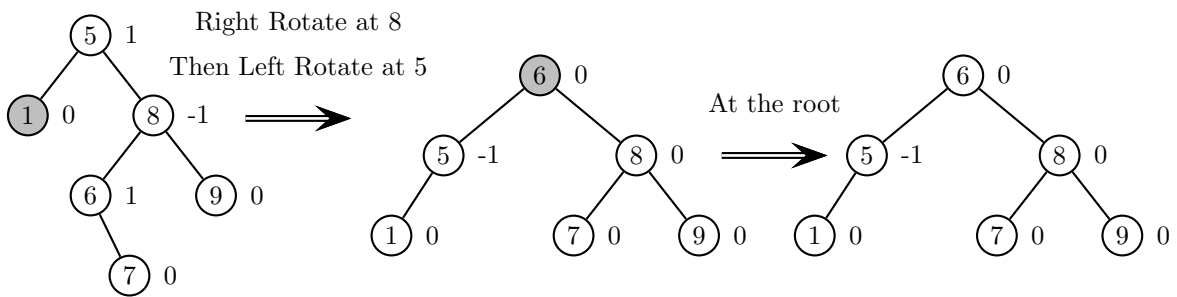
Figure 24.15: Removing 4.
