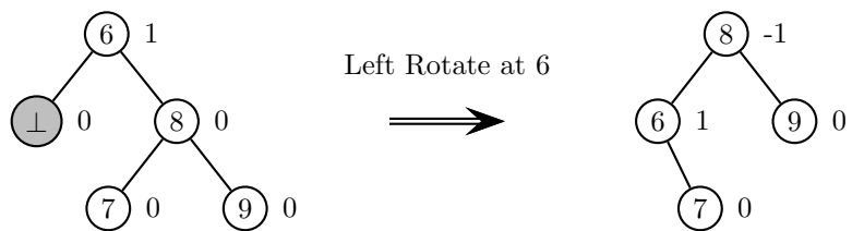
Figure 24.16: Removing 1, then 5.
