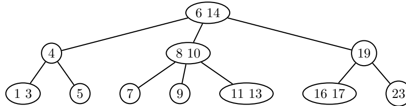
Figure 25.13: The tree T with the key 16 added.
