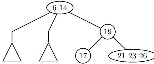
Figure 25.3: After inserting the key 26. Having three keys in a node is illegal, so we need to fix this.
