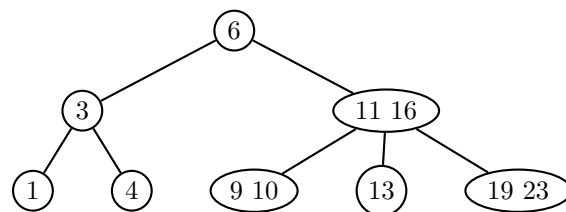
Figure 25.24: Borrowing from the parent to resolve the empty node in the middle of the tree.
