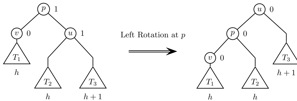
Figure 24.12: When b(u) = 1 , a single left rotation at p fixes the local problems, but the height of the subtree shrunk, so we need to recurse to higher levels.
